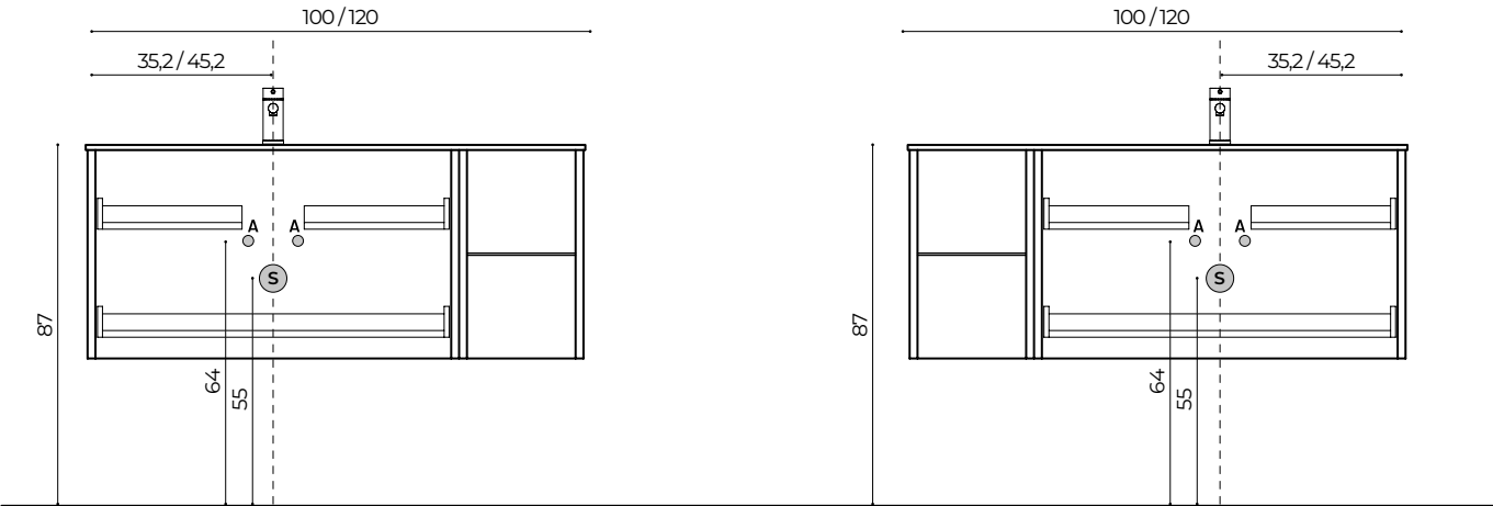
QUOTE BASI PORTALAVABO DECENTRATE CON LAVABO L.100 (70+30)/L.120 (90+30) H.1,3 (ES. FIANCHI H.50) QUOTAS DISCHARGES DECENTRALIZED BASE UNIT FOR WASHBASIN WITH WASHBASIN W.100 (70+30) / W.120 H.1,3 (EX. SIDES H.50)
