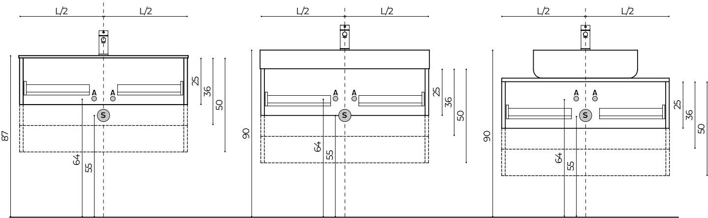
QUOTE BASI PORTALAVABO CX H.25, H.36, H.50 QUOTAS DISCHARGES BASE UNIT FOR WASHBASIN CX H.25, H.36, H.50
