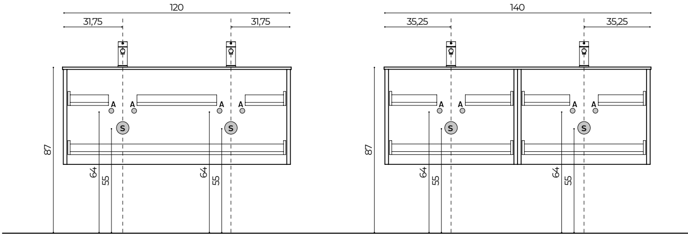
QUOTE BASI PORTALAVABO DOPPIA VASCA CON LAVABO H.1,3 (ES. FIANCHI H.50) QUOTAS DISCHARGES BASE UNIT FOR WASHBASIN WITH DOUBLE BASIN WASHBASIN H.1,3 (EX. SIDES H.50)
