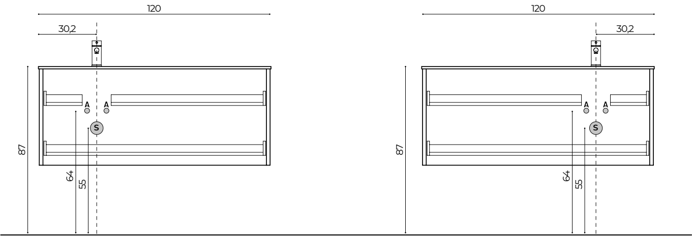
QUOTE BASI PORTALAVABO DECENTRATE CON LAVABO L.120 H.1,3 (ES. FIANCHI H.50) QUOTAS DISCHARGES DECENTRALIZED BASE UNIT FOR WASHBASIN WITH WASHBASIN W.120 H.1,3 (EX. SIDES H.50)
